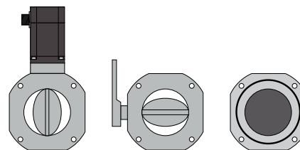
Throttle body for engines with existing sealing on flange
